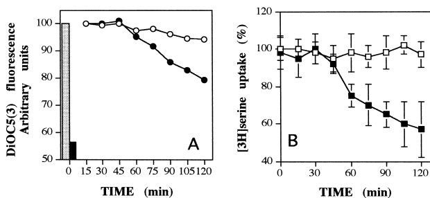
Fig. 4. CD95 induces a late plasma membrane depolarization and a decreased uptake of [ ^3\text{H} ]serine. Jurkat cells (A) were left untreated ( \circ ) or treated with CD95 (0.5 \mu\text{g}/\text{ml} ) ( \bullet ) for different periods of time and the membrane potential was measured by cytofluorimetry with the DiOC5(3) probe. The bars on the left of the figure show the polarization status of the cells at time 0 and after 15 min of treatment with 1 \mu\text{M} gramicidin. B: The total uptake of [ ^3\text{H} ]serine by the cells was measured as a function of time. Each point is the mean \pm S.D. of triplicate determinations from a typical experiment.
